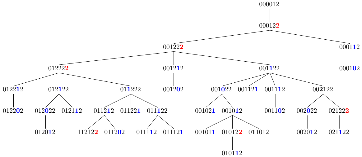
■ Figure 3 The cycle-joining tree T_3(6) . Each node differs from its parent (cyclically) at the highlighted symbol. The symbols highlighted in blue indicate that \text{par}(\alpha) = \text{lastNonMax}(\alpha) ; the symbols highlighted in red indicate that \text{par}(\alpha) = \text{lastSymbol}(\alpha) ; the symbols highlighted in bold black indicate that \text{par}(\alpha) = \text{firstNonMin}(\alpha) . There are no nodes in this tree such that \text{par}(\alpha) = \text{secondLastNonMax}(\alpha) ; the first instance of such a case arises when n = 12 .
